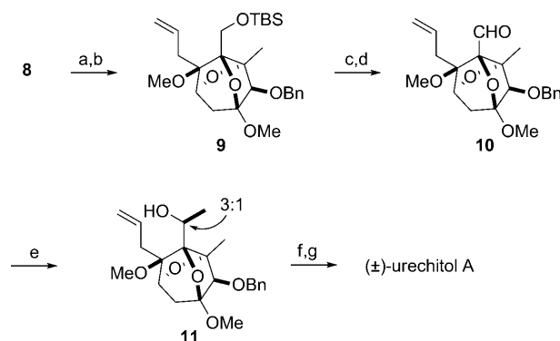
Scheme 4. a) Allylmagnesium bromide, THF, 0 °C, 73 %; b) NaH, MeI, THF, 0 °C–RT, 87 %; c) TBAF, THF, RT, 92 %; d) TPAP, NMO, M.S. 4 Å, \text{CH}_2\text{Cl}_2 , RT, 92 %; e) MeMgCl, THF, 0 °C–RT, 67 % of 11 and 24 % of the stereoisomer; f) \text{OsO}_4 , NaIO 4 , 2,6-lutidine, dioxane/ \text{H}_2\text{O} , RT, 67 %; g) \text{H}_2 , Pd(OH) 2 , EtOH, RT, 87 %. THF = tetrahydrofuran, TBAF = tetra- n -butylammonium fluoride.
